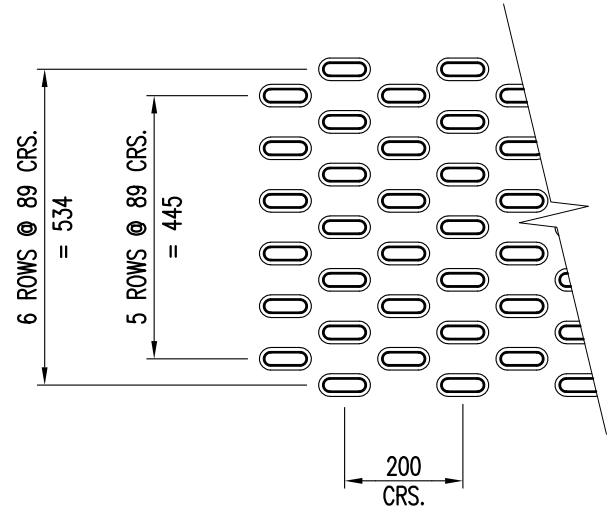
TYPE '4' 70 x 20 OBROUND FORMUP
