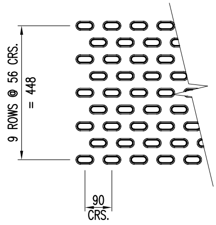
TYPE '2' 50 x 20 OBROUND FORMUP
