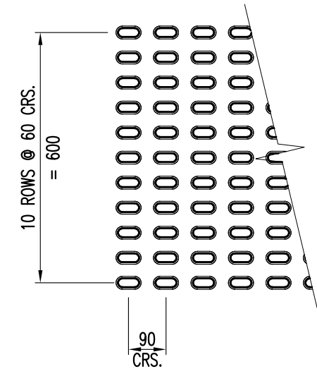
TYPE '3' 50 x 20 OBROUND FORMUP
