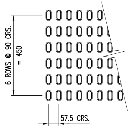
TYPE '1' 50 x 20 OBROUND FORMUP
